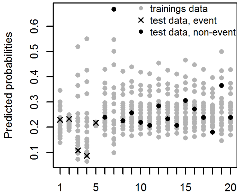
Maximum likelihood
