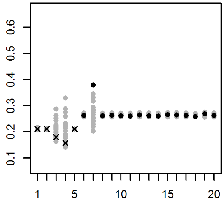
Ridge
